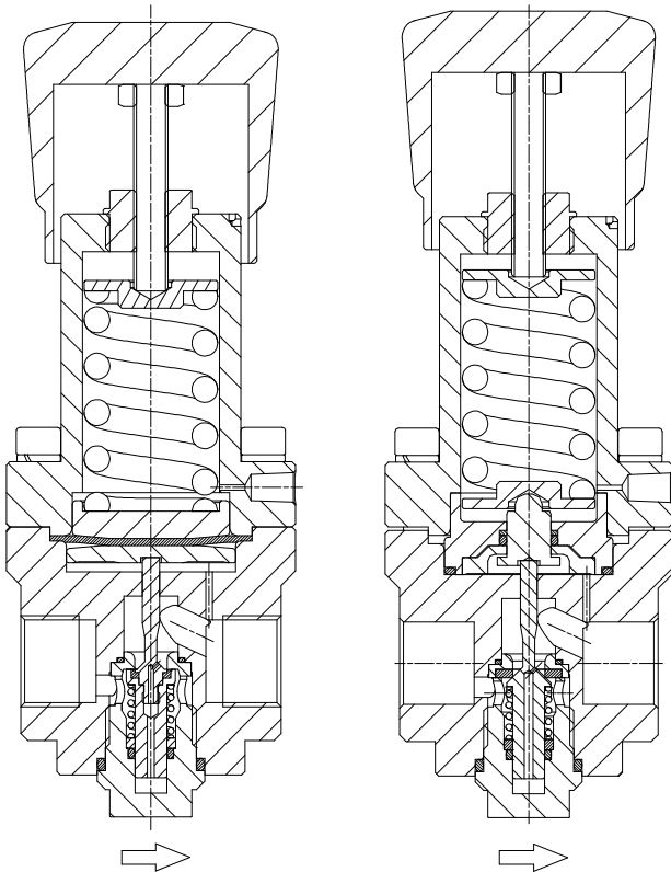
Section view of: GRT20S-50B8-SSNN
