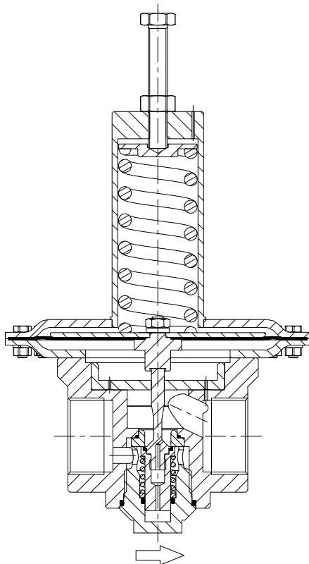
Section view of: GRT40S-16N1-SSW
